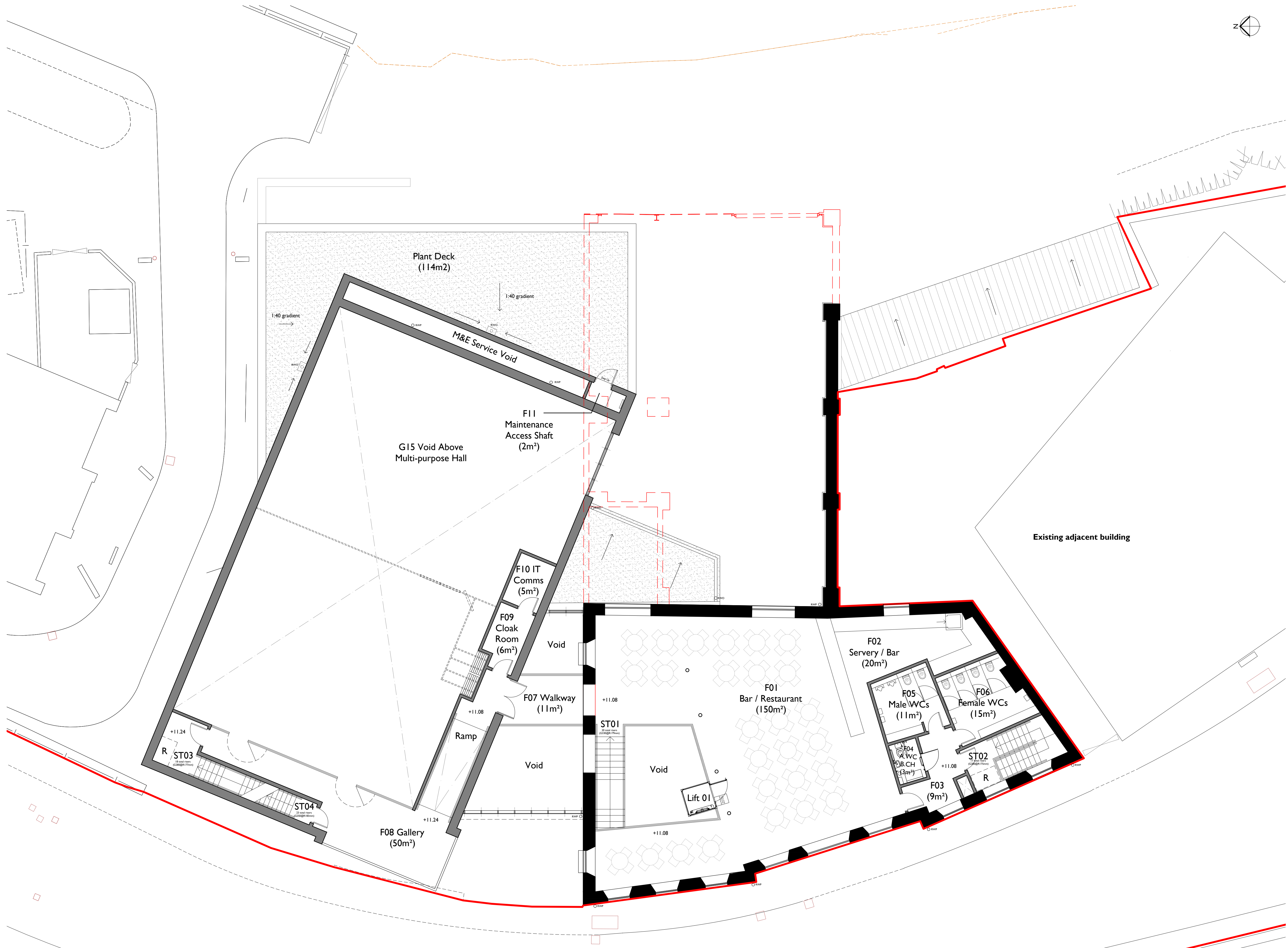
I Proposed First Floor Plan 2101 1:100 at A1
